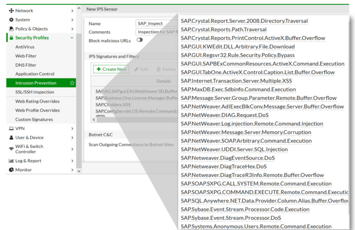
Figure 13: Sample of IPS Signatures for SAP
