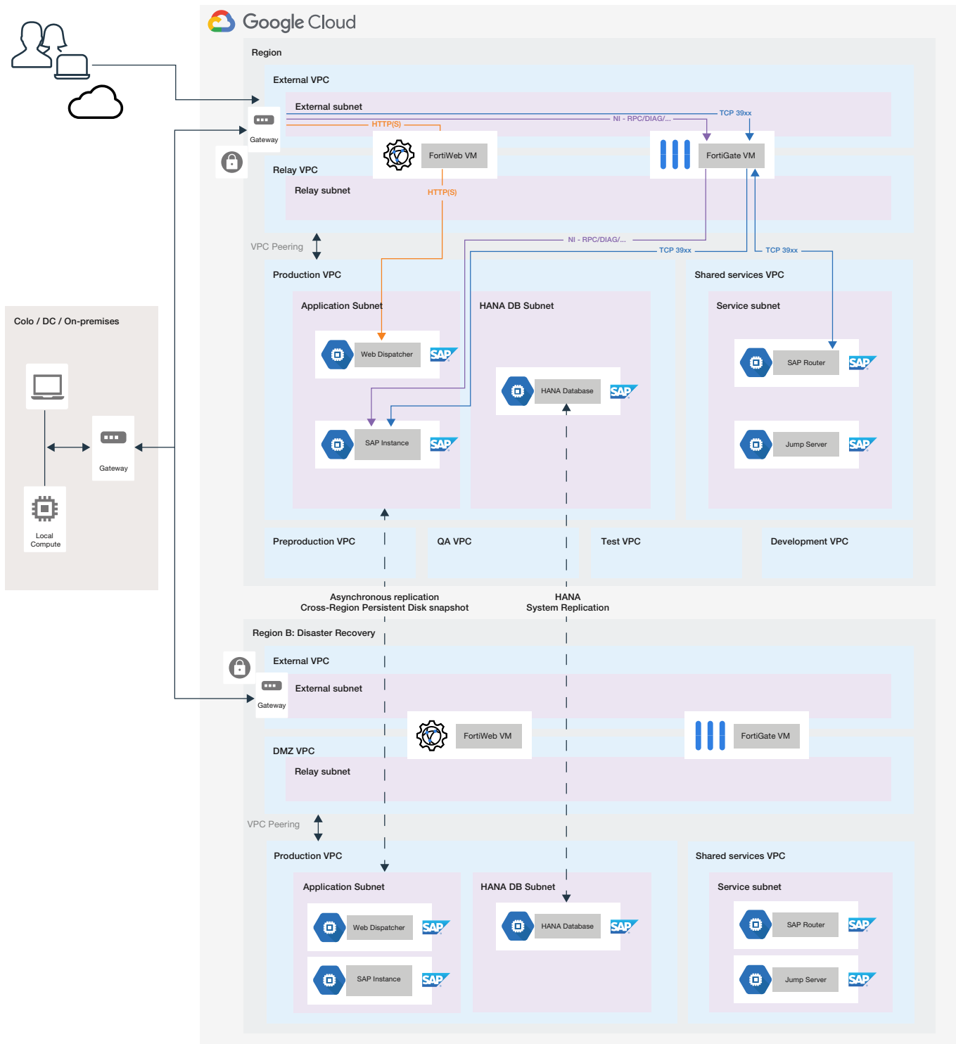
Figure 23: Fortinet Reference Architecture for SAP S/4HANA on Google Cloud with disaster recovery
