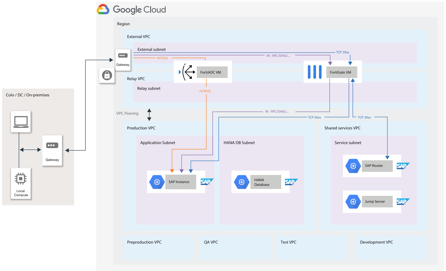
Figure 22: Fortinet Reference Architecture for SAP S/4HANA on Google Cloud
