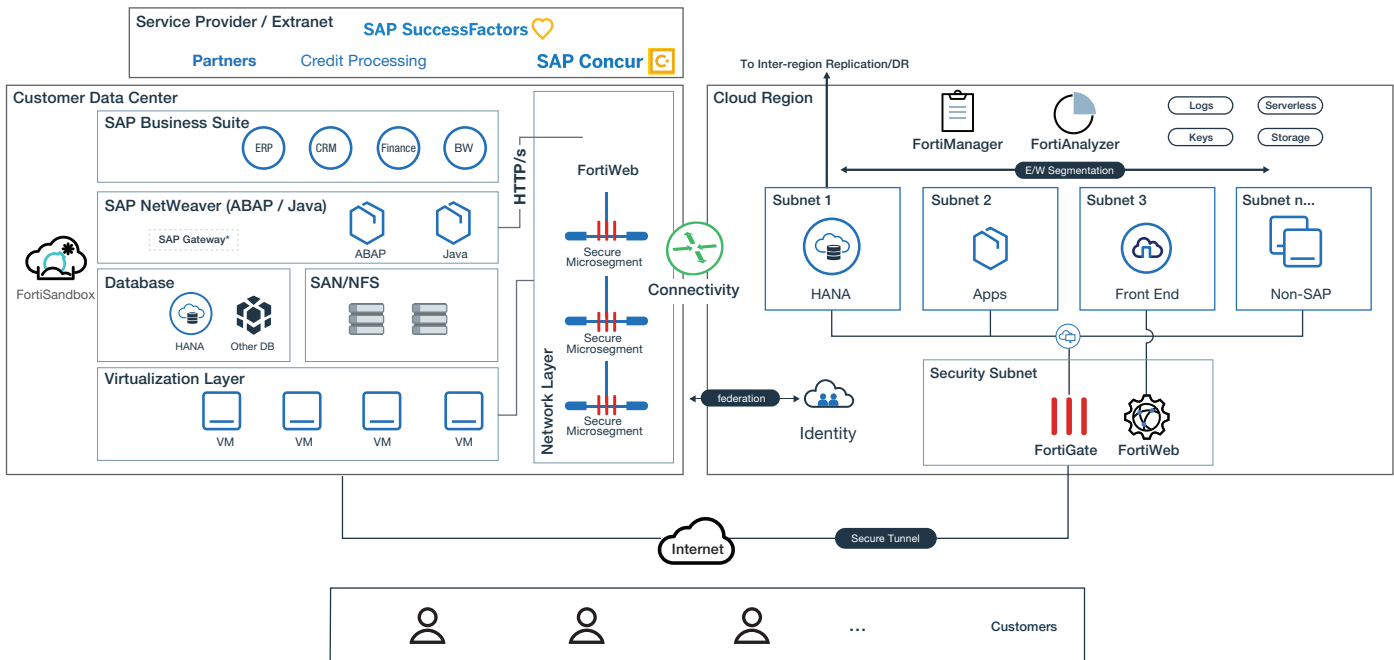
Figure 24: Fortinet Reference Architecture for SAP S/4HANA in Hybrid Environment
