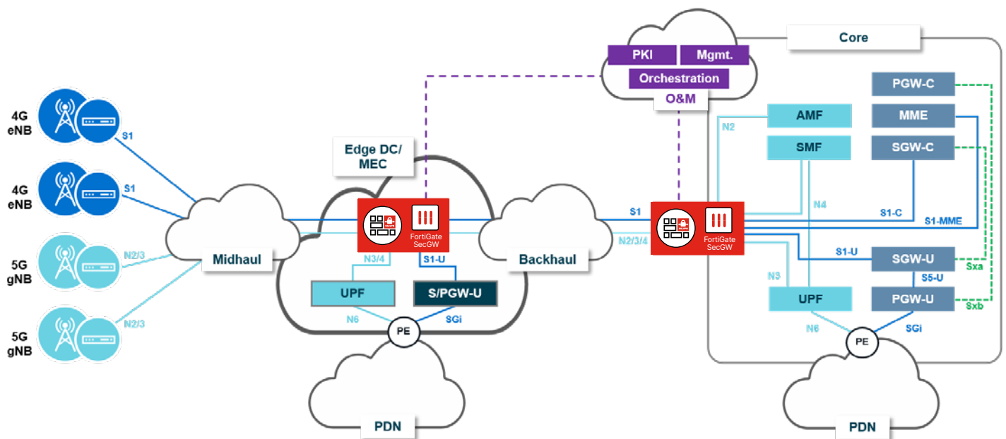
FIGURE 3: DISTRIBUTED SEC GW WITH EDGE CLOUD DEPLOYMENT
