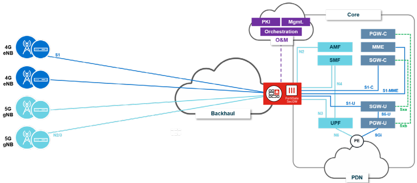
FIGURE 2: CENTRALIZED SEC GW DEPLOYMENT
