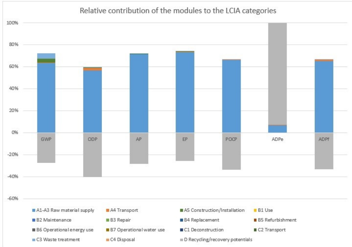
Fig. 1: Environmental impact of aluminium sliding shutters along the lifecycle (impact of production modules A1–A3 = 100 %)
