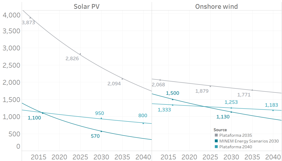
Figure 3 Investment costs projections for onshore wind and solar PV. The gray cost curve represents pre-NDC cost expectations and the blue curves post-NDC cost expectations.
