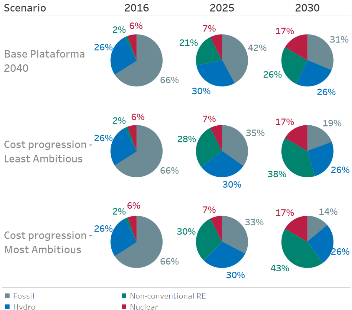
Figure 7 Evolution of power generation shares in Argentina in base case scenario and under least and most ambitious cost progression scenarios.
