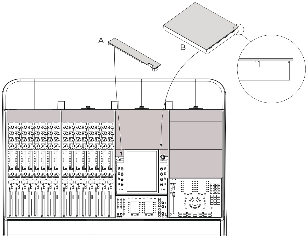
Figure 1. Master Compression Panel and Frame Panel Large Center in a Frame Chassis Small
